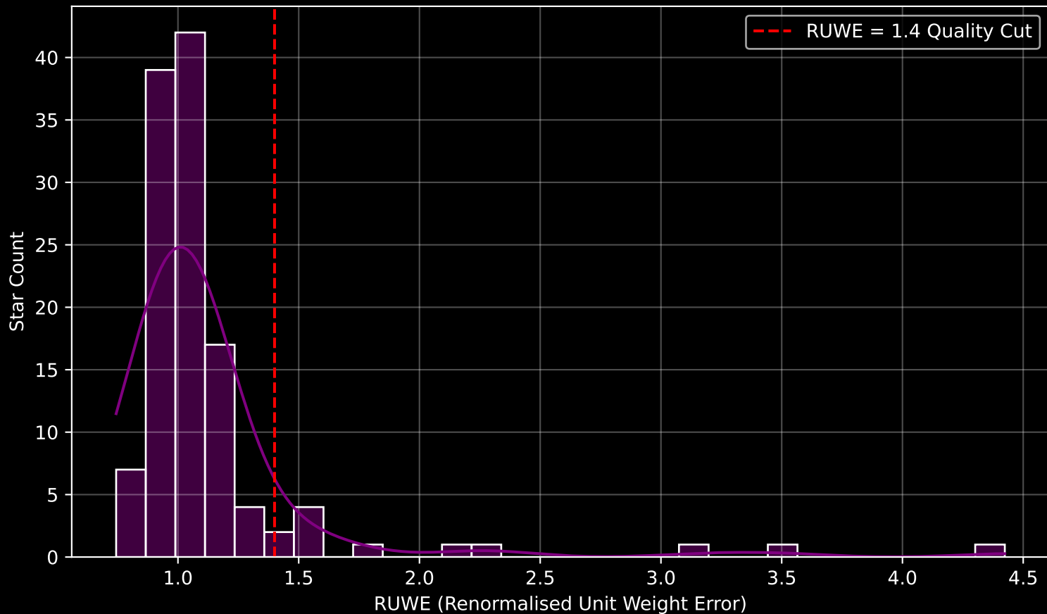
GALAH DR4 Field [7212] RUWE Distribution (n= 121)
