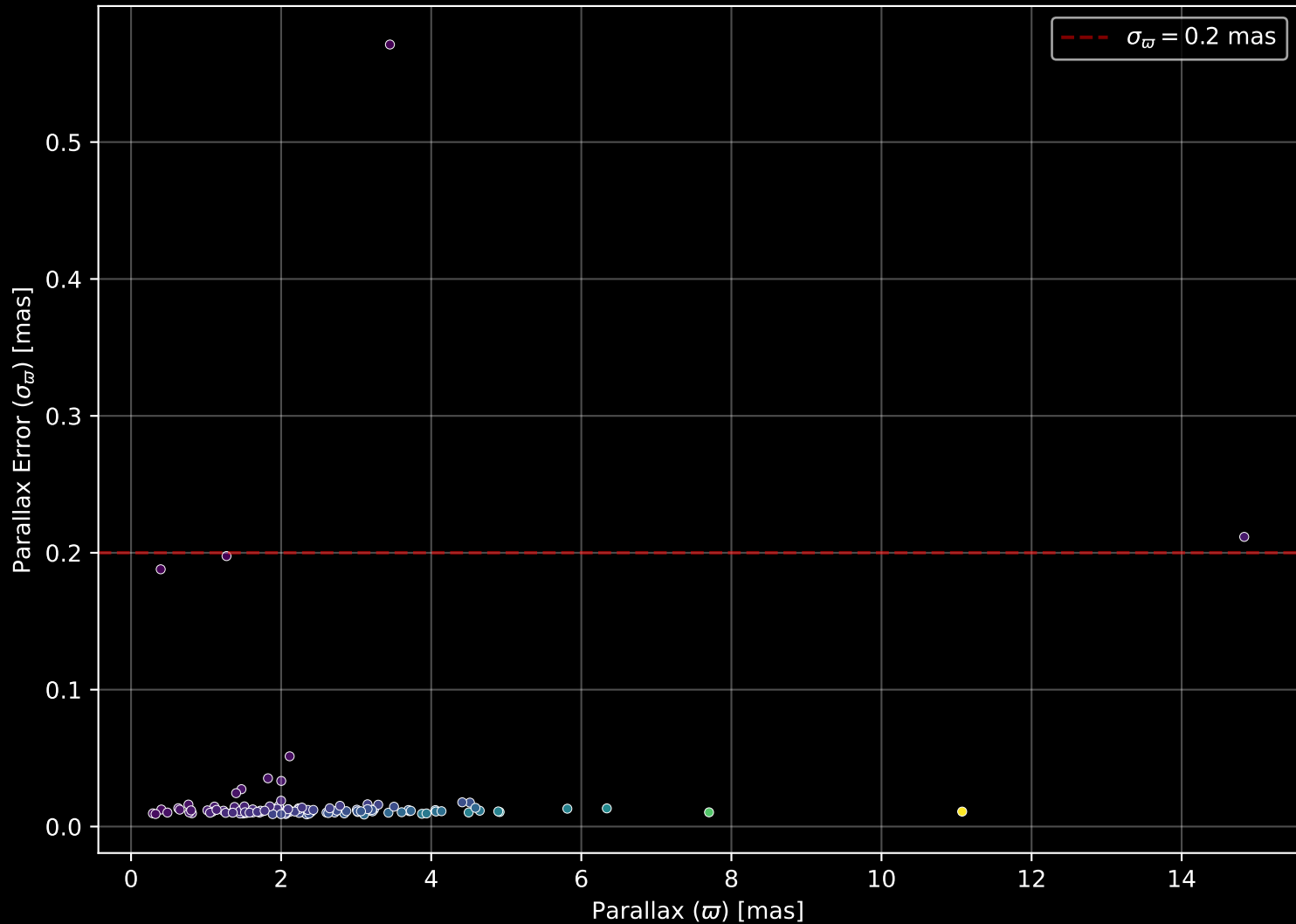
GALAH DR4 Field: [7212] Parallax Quality (n= 125)
