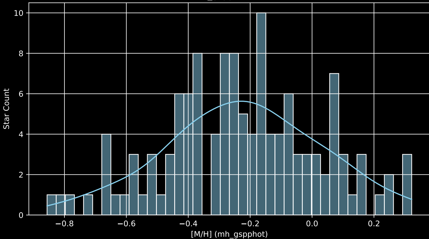
GALAH DR4 Field: [7212] [M/H] (mh_gspphot) (n= 125)
