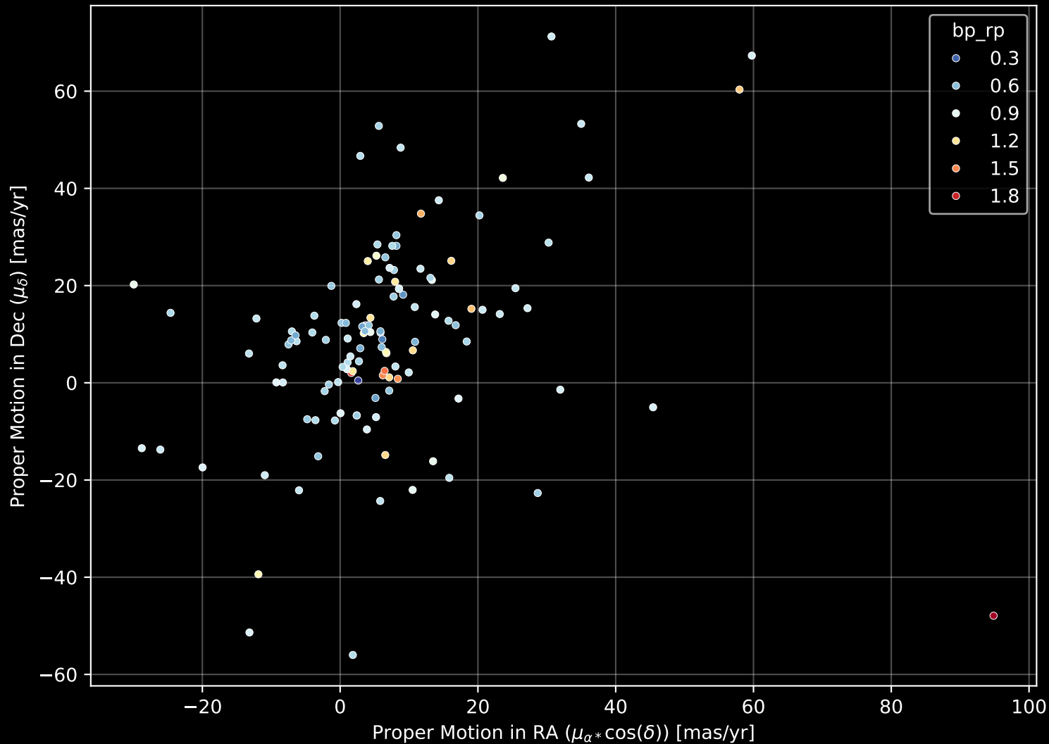
GALAH DR4 Field: [7212] Proper Motion Diagram (n= 125)
