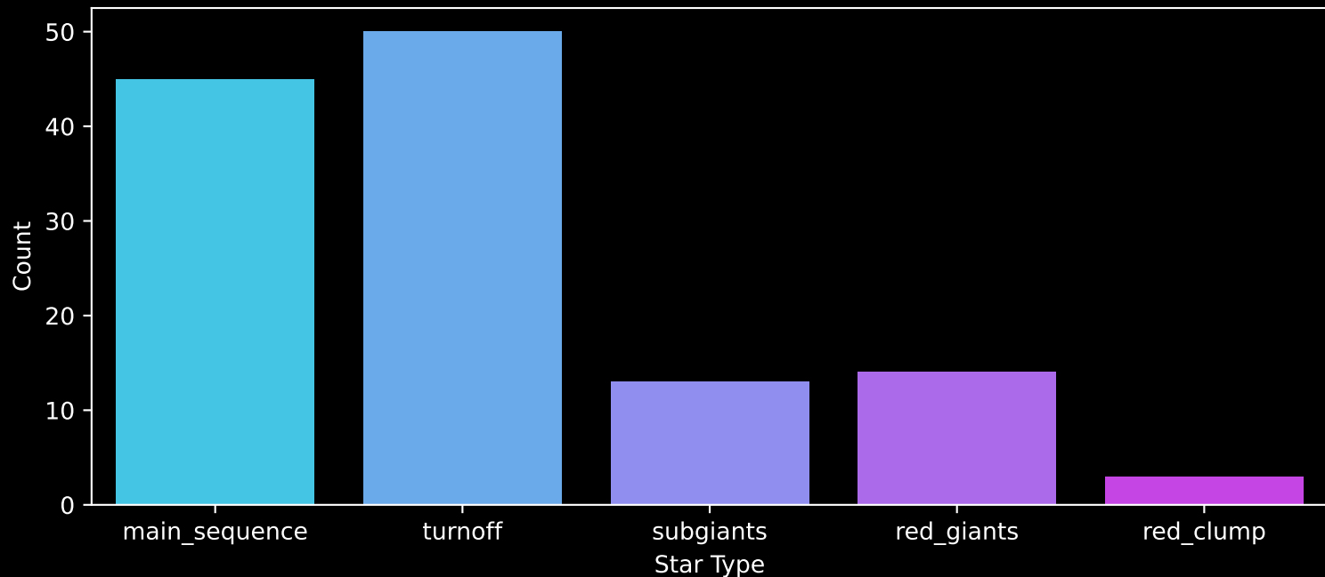
GALAH DR4 Field: [7212] Count plot of Star Type
